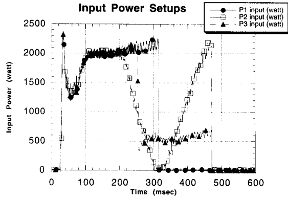
Fig. 1. Temporal behavior of input microwave power. Three different profiles are used throughout the experiments and denoted as P1, P2 and P3.
